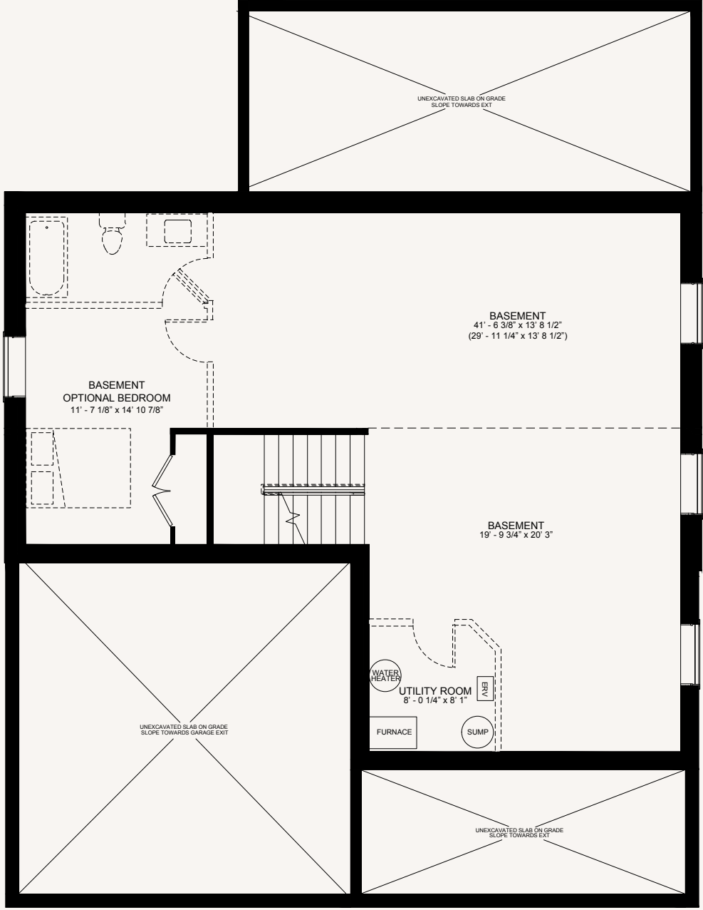
OPTIONAL FINISHED BASEMENT 1154 SQ.FT.
